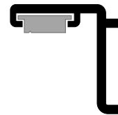
#3389 SC-551(64713)/V-253 Strike Jamb Assy
