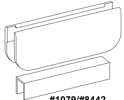
#1079/#8442 1038/1090 Top/Bottom Door Rail w/V-296
