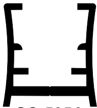
SC-505A 63235 Curb with weep slots
