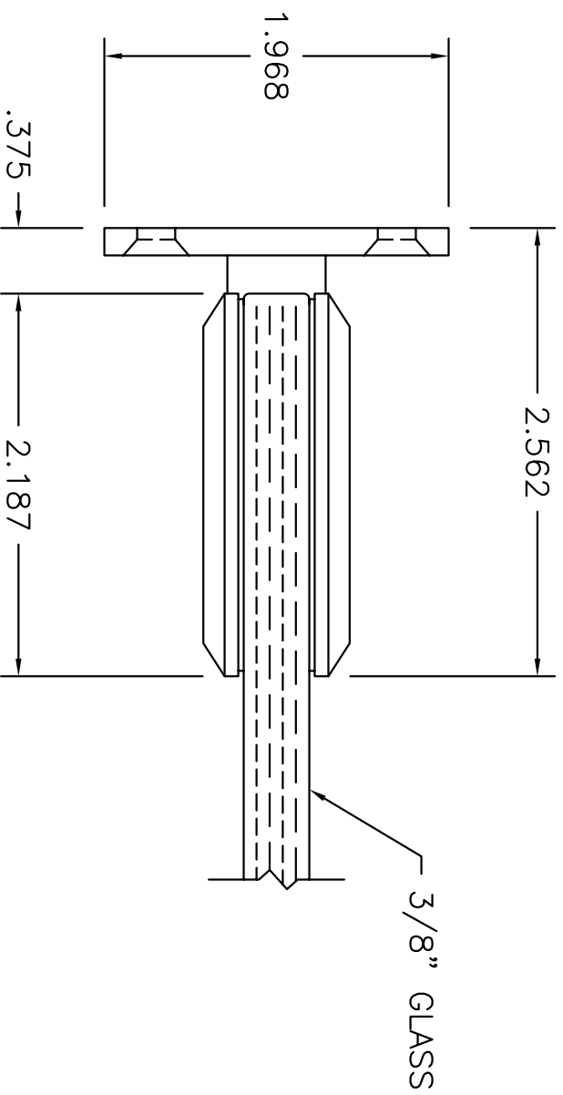
TOP VIEW OF HINGE AND GLASS FULL SIZE
