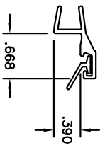
EPH-N00-04830 3/8" 180° STRIKE & DOOR JAMB
