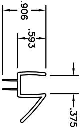
EPH-N00-04829 3/8" BOT. W/DRIP
