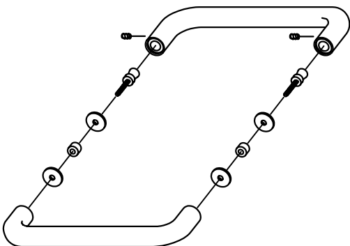
6" TUBULAR BACK TO BACK HANDLE
