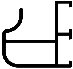
SC-554 64853 Mirror Frame
