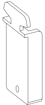
#4339 Header T-Lock for 1040
