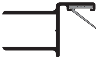
SC-552 64520 w/V-314 Strike Jamb 1-5/8" x 1"
