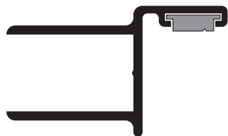
SC-552 64520 w/4033 Strike Jamb 1-5/8" x 1"
