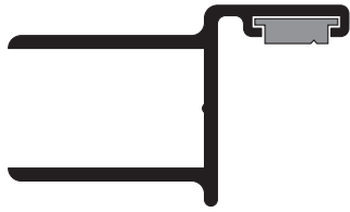
SC-552 64520 w/4033 Strike Jamb 1-5/8" x 1"
