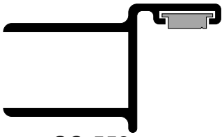
SC-552 64520 w/V-253 Strike Jamb 1-5/8" x 1"
