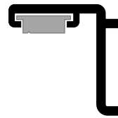
SC-551 (64713)/V-253 Strike Jamb Assy 13/16" x 13/16"
